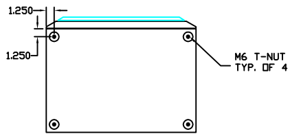
(I) BOTTOM VIEW
