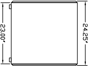
3 FRONT VIEW
